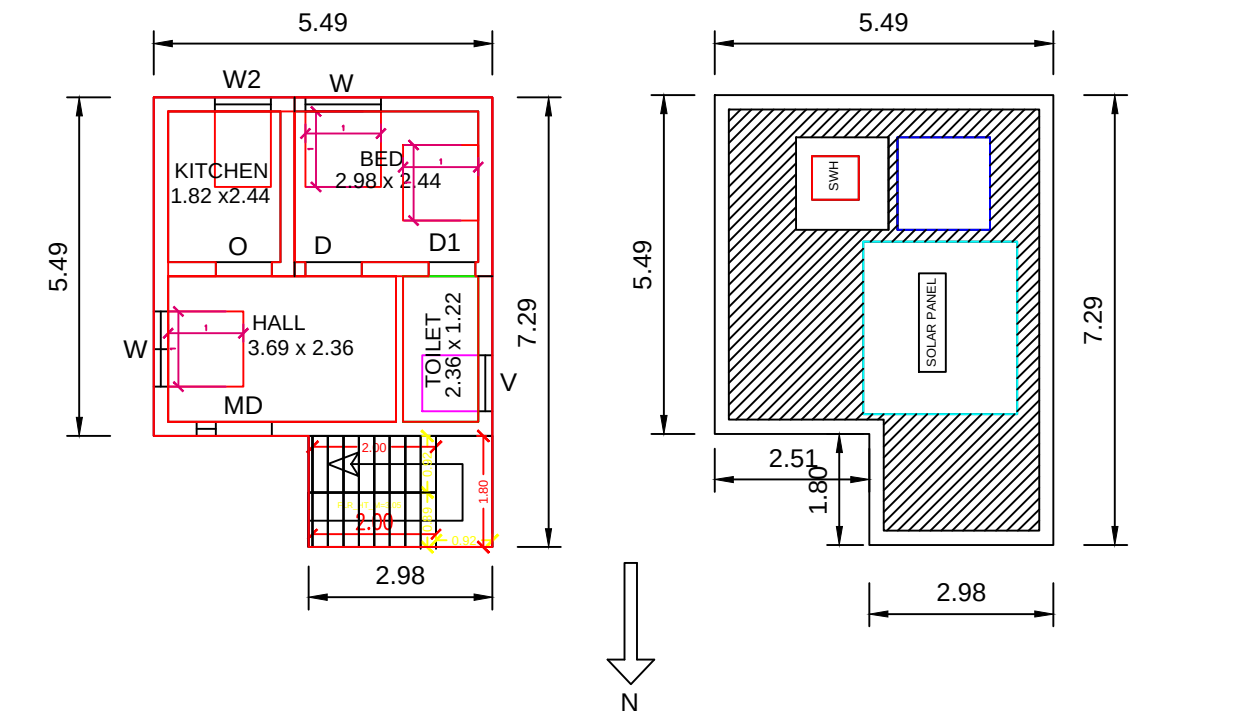
GROUND FLOOR PLAN TERRACE FLOOR PLAN
