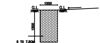
SECTION OF PEBBLE TRENCH
