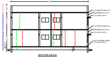
SECTION ON B-B
