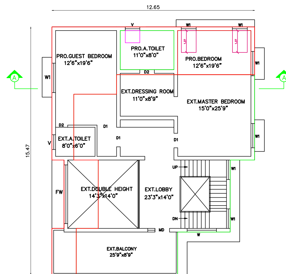
EXISTING & PROPOSED FIRST FLOOR PLAN
