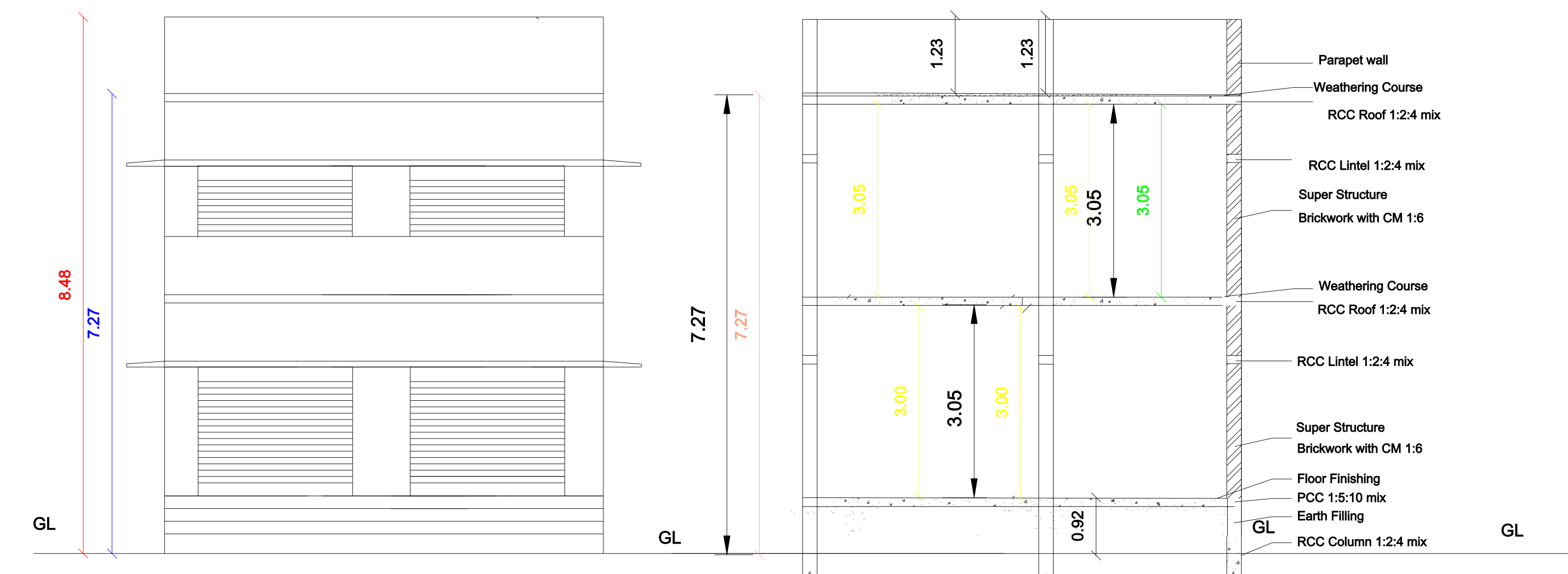
FRONT ELEVATION
