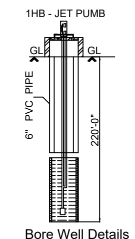
Bore Well Details
