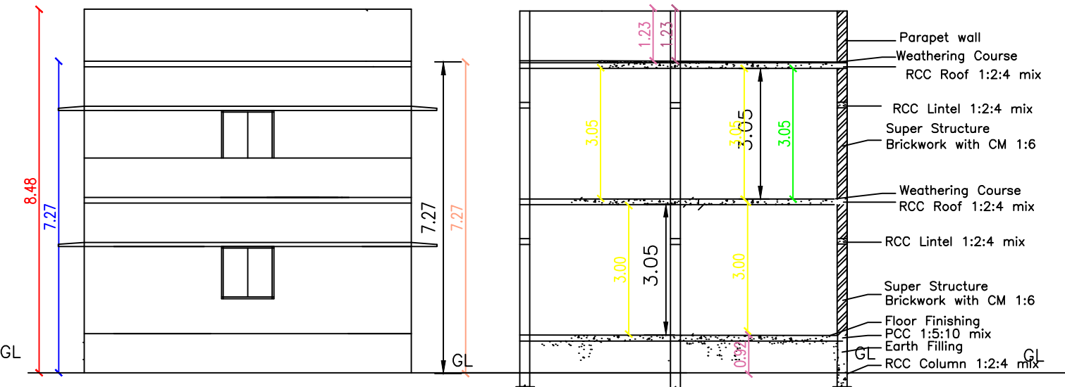
FRONT ELEVATION
