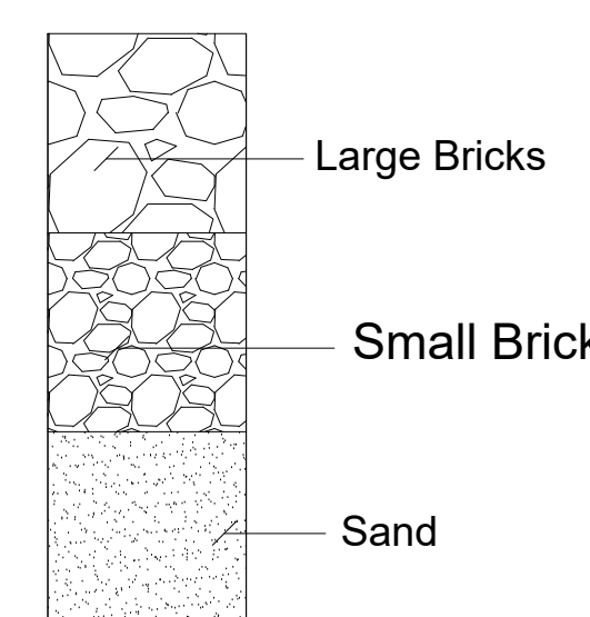
SECTION OF RAIN WATER COLLECTION PITS (NTS)
