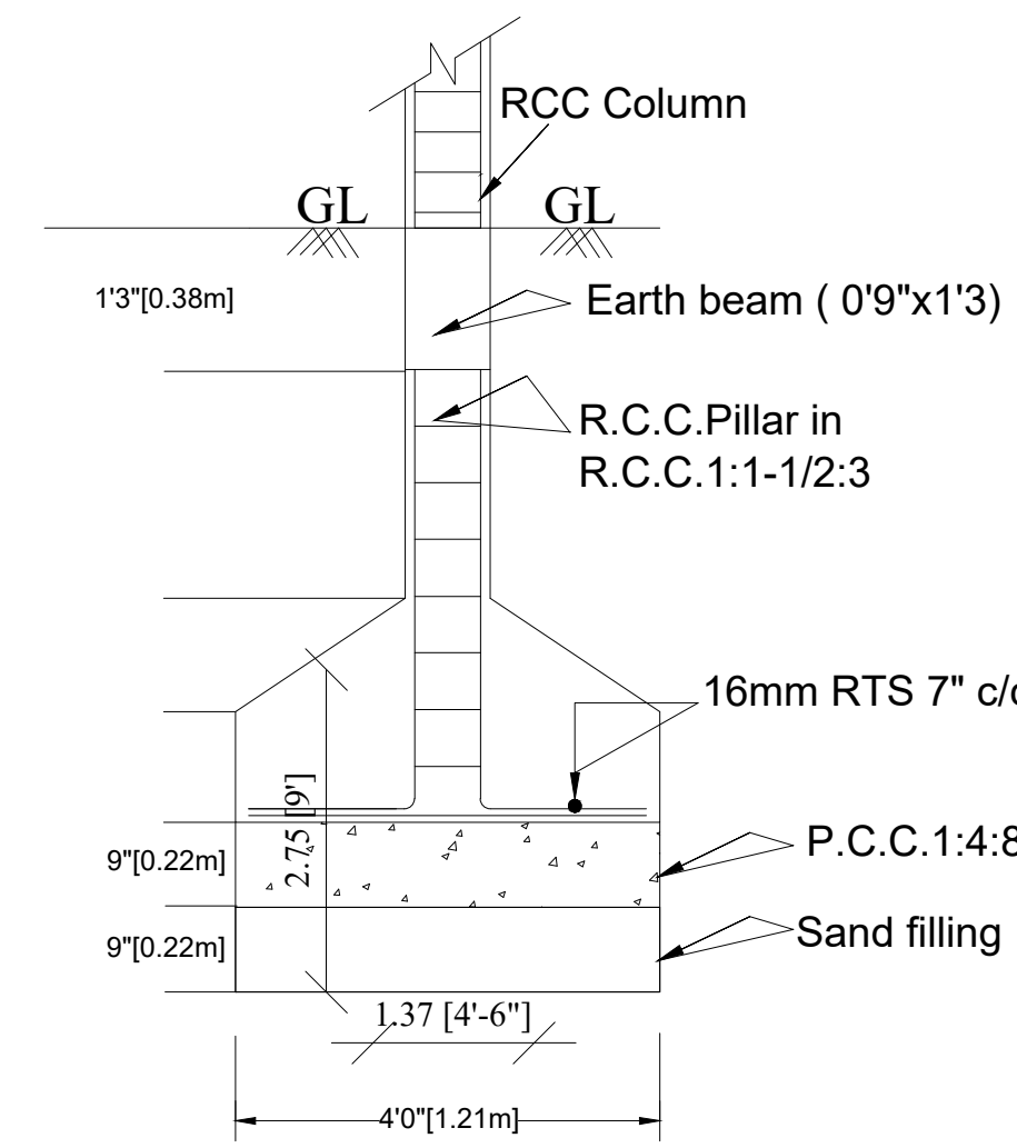
FOUNDATION DETAILS
