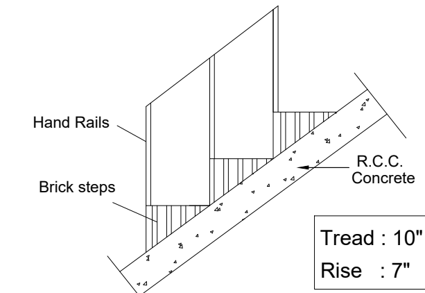
STAIRCASE DETAILS
