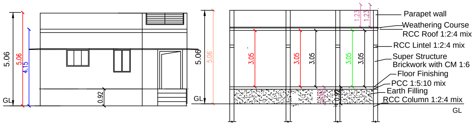
FRONT ELEVATION
