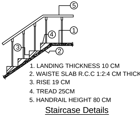
Staircase Details
