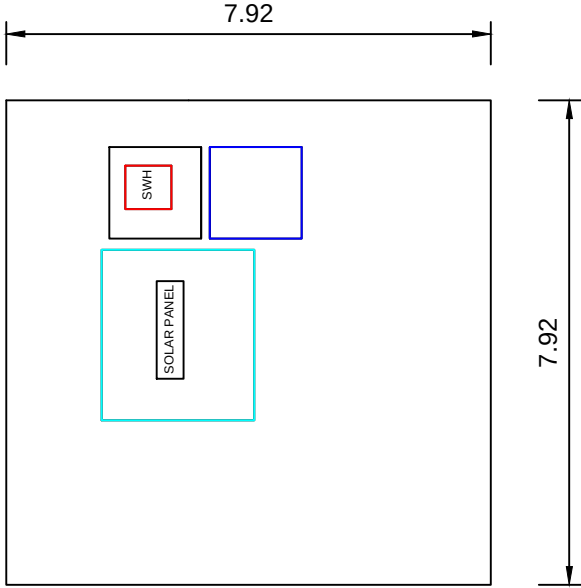
TERRACE PLAN
