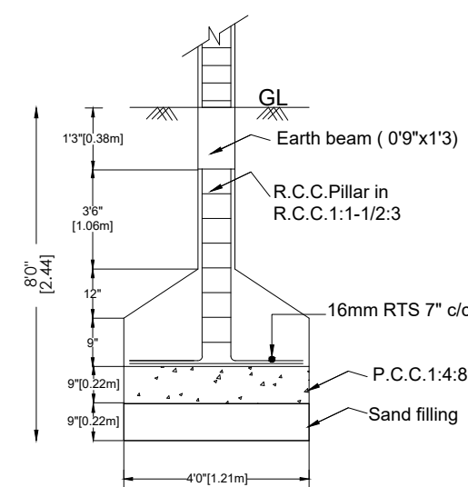
FOUNDATION DETAILS
