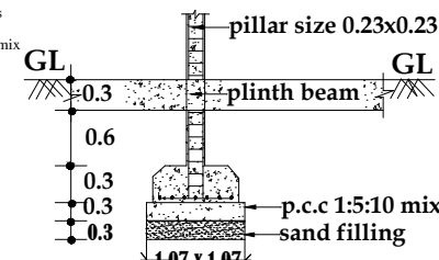
FOUNDATION DETAILS
