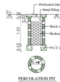
PERCOLATION PIT
