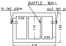
SEPTIC TANK PLAN
