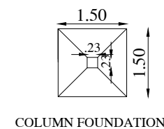
COLUMN FOUNDATION
