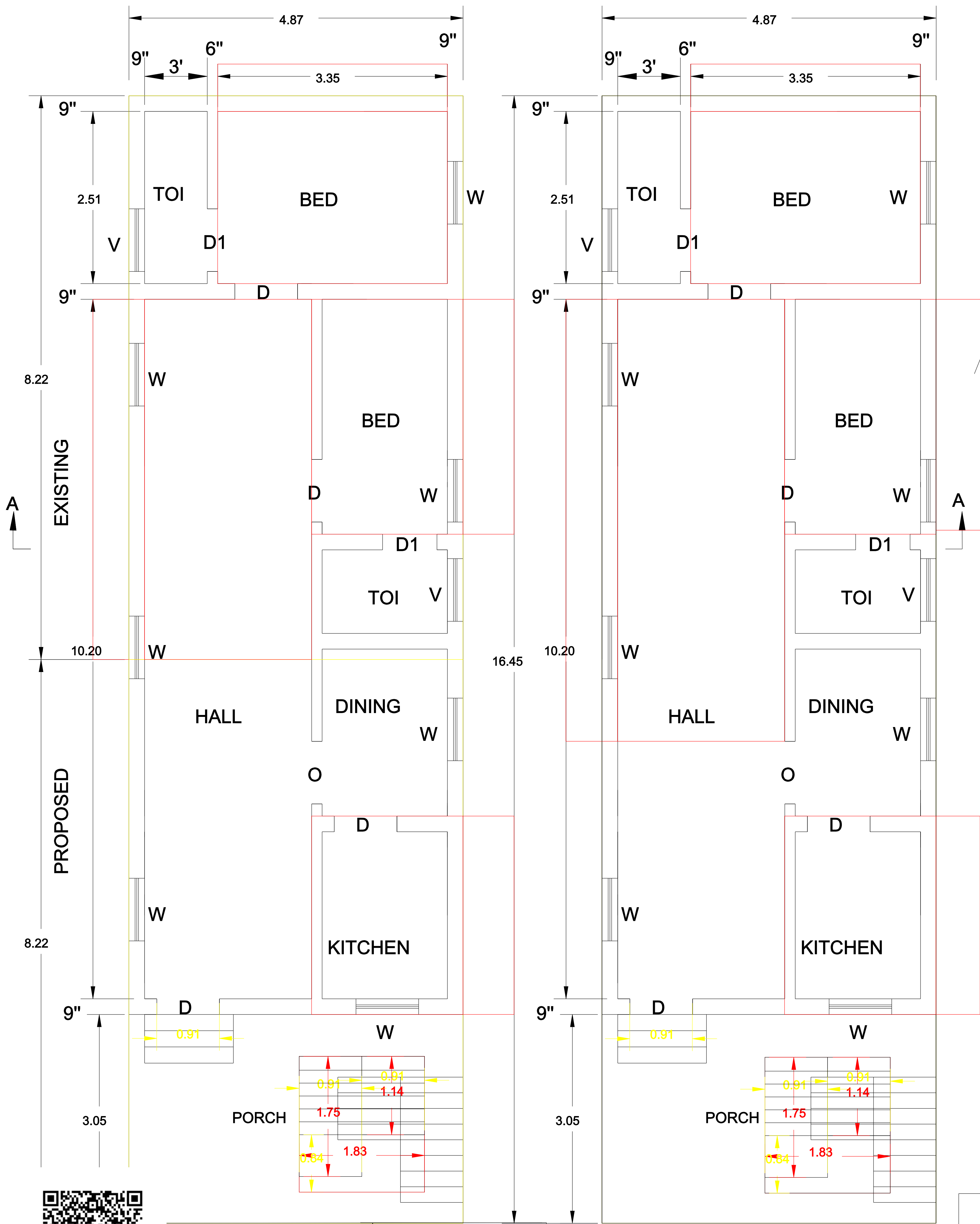
G.F. PLAN
