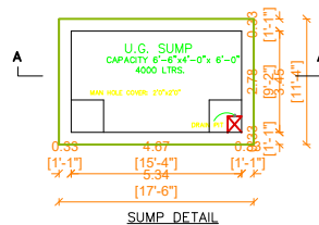
SUMP DETAIL
