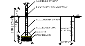
FOUNDATION DETAILS-MIDDLE COLUMN
