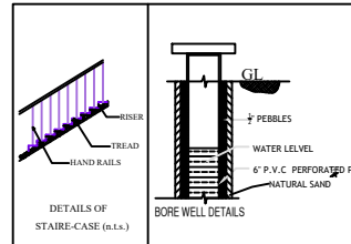
DETAILS OF STAIRCASE (in L.S.)
