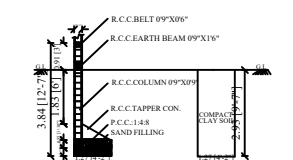
FOUNDATION DETAILS-END COLUMN
