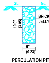
PERCULATION PIT
