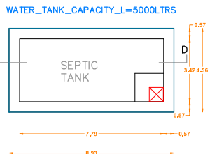
PLAN OF SEPTIC TANK SCALE 1"=2'0"
