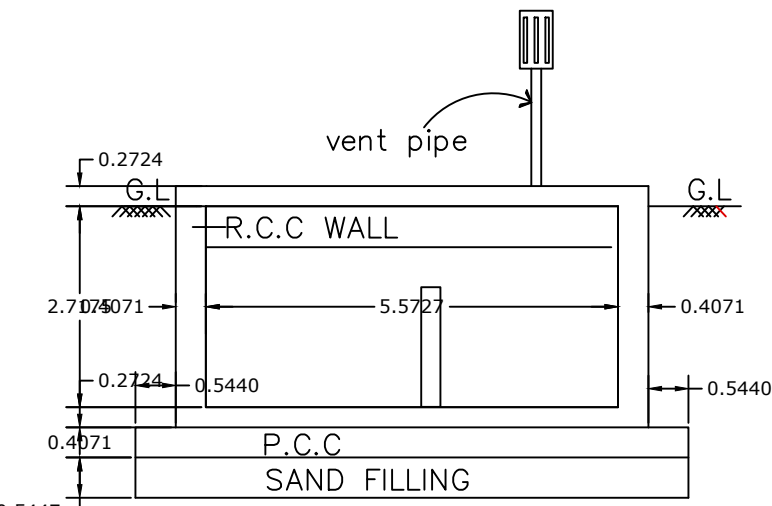
SECTION ON D-D
