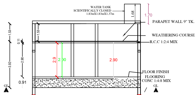
SECTION ON "M-L"
