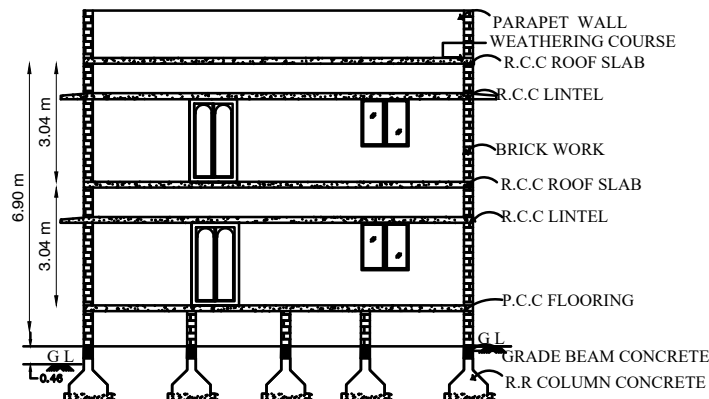
SECTION ON X X
