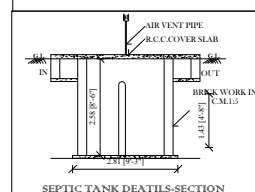
SEPTIC TANK DETAILS-SECTION
