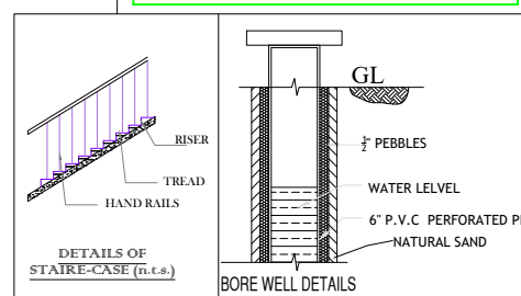
BORE WELL DETAILS
