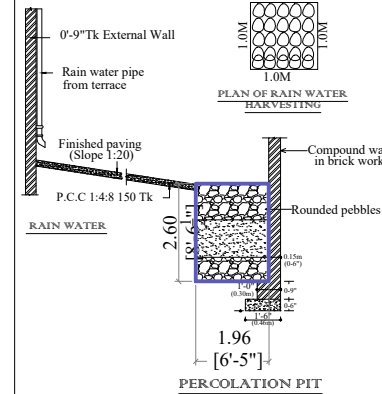
PERCOLATION PIT
