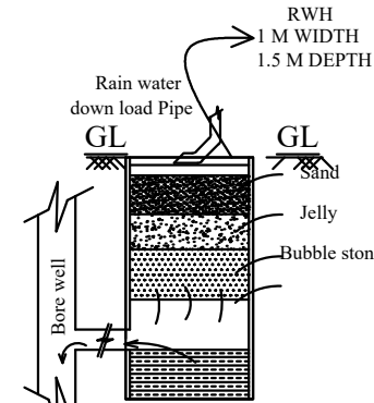
SEC. RAIN WATER HARVEST PIT
