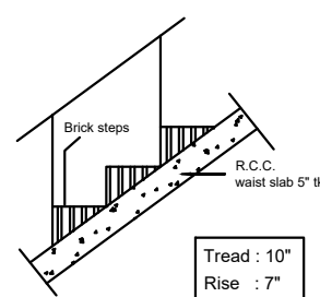
STAIRCASE DETAILS-N.T.S
