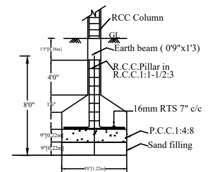
FOUNDATION DETAILS
