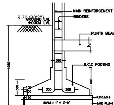
TYPICAL SECTION OF R.C.C. COLUMN FOUNDATION
