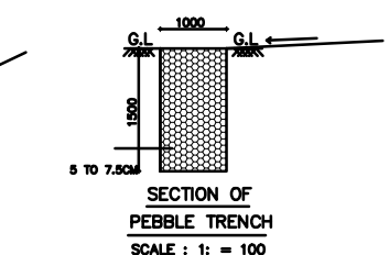
SCALE : 1: = 100
