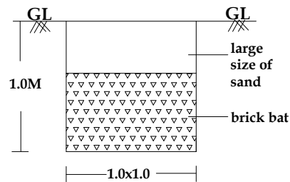
RAINWATER HARVESTING
