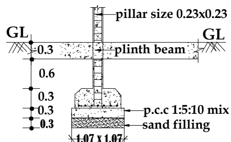
FOUNDATION DETAILS
