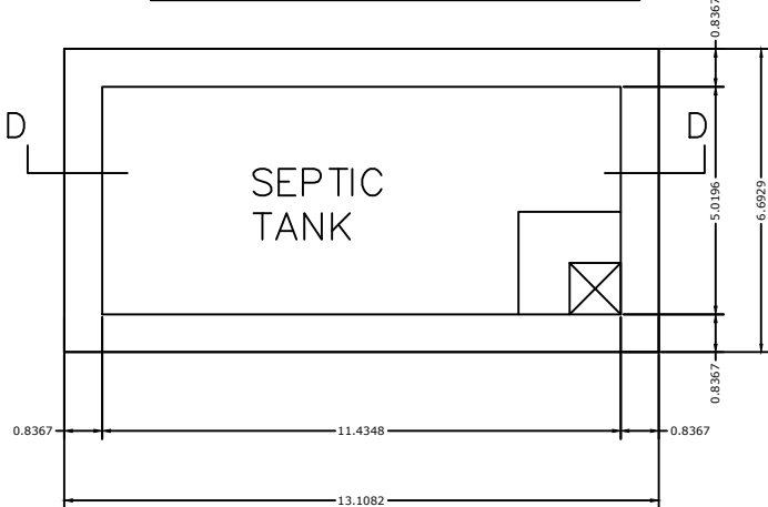
PLAN OF SEPTIC TANK SCALE 1" = 2'0"
