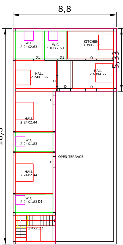
SECOND FLOOR PLAN (PROPOSED)
