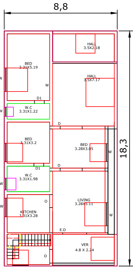
FIRST FLOOR PLAN (EXISTING) (PROPOSED)
