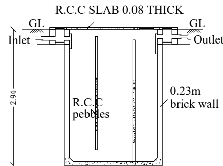
SECTION OF SEPTIC TANK
