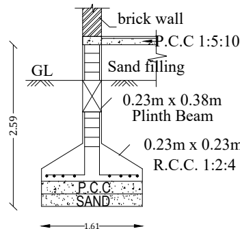
FOUNDATION DETAILS
