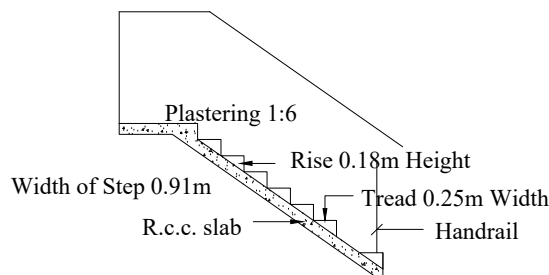
DETAILS OF STAIR CASE
