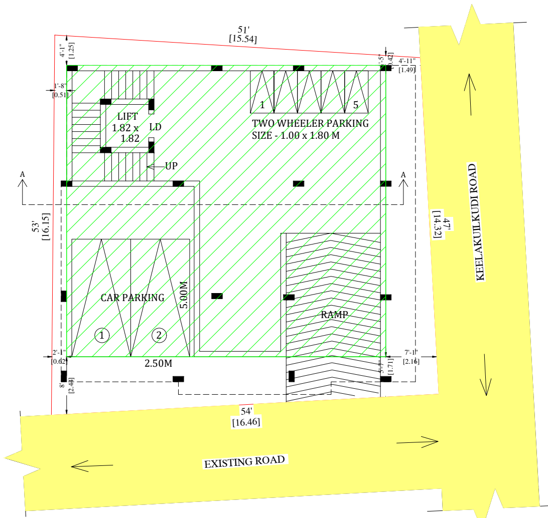
EXISTING BASEMENT FLOOR PLAN
