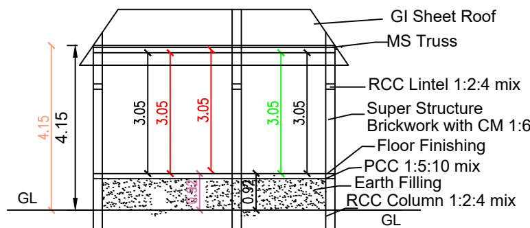
SECTION ON "VR"
