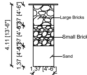
SECTION OF RAIN WATER
