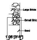
SECTION OF RAIN WATER COLLECTION PITS (NTS)
