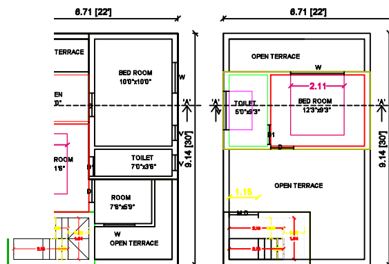
PRO. SECOND FLOOR PLAN
