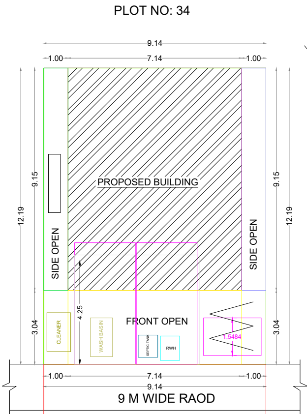
SITE PLAN
