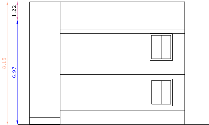
ELVATION
