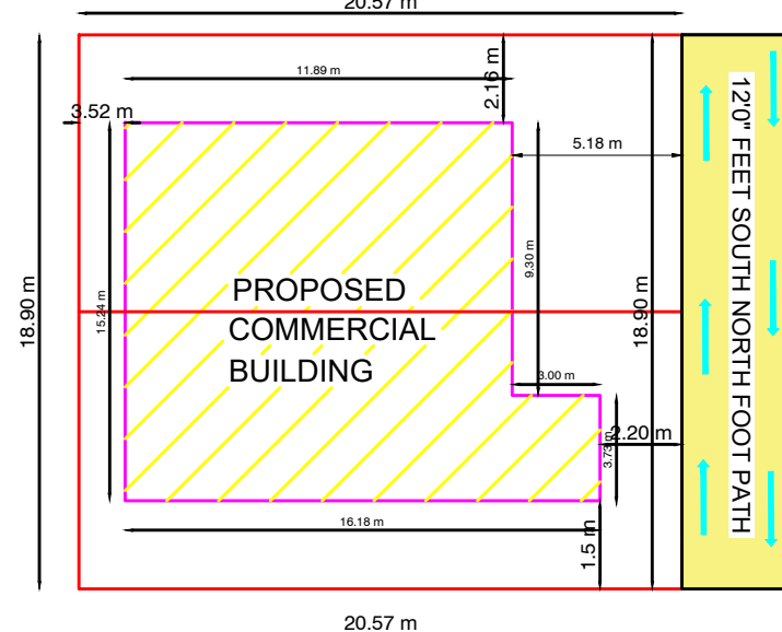
RAMASAMY'S LAND SITE PLAN (NTS)
