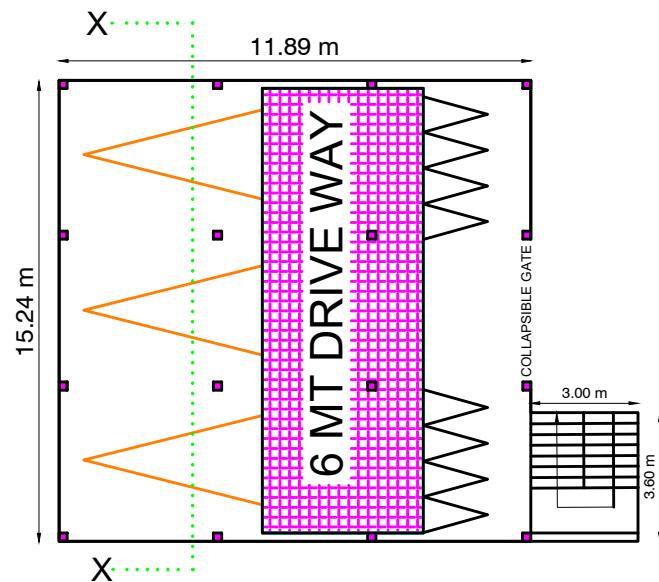
PROPOSED STILT FLOOR PLAN
