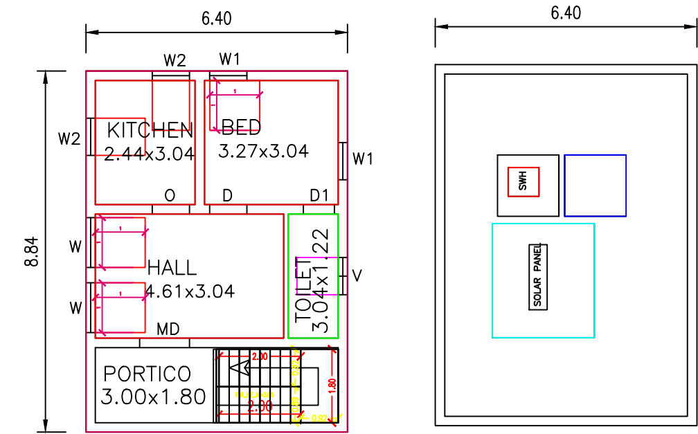
GROUND FLOOR PLAN TERRACE PLAN
