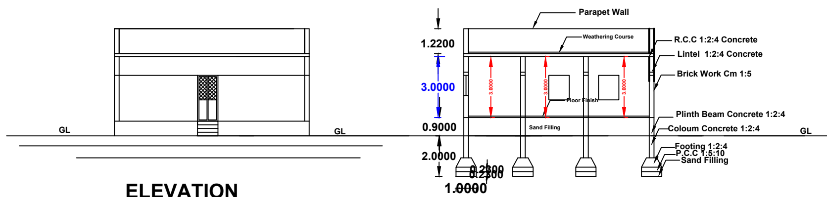
Section - AA
