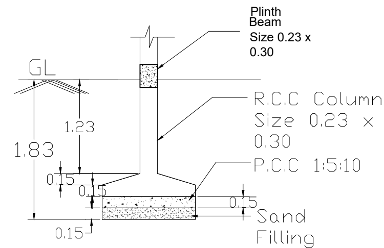
FOUNDATION DETAILS
