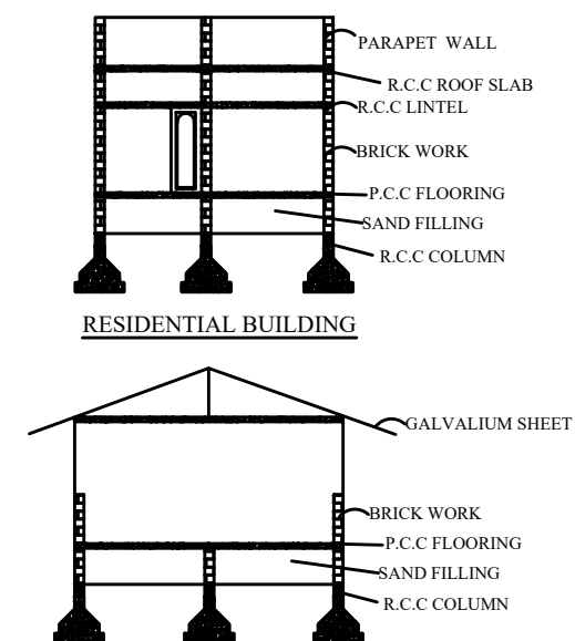
SHED 1 & 2 SECTION ON X- X
