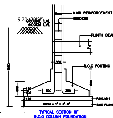
TYPICAL SECTION OF R.C.C COLUMN FOUNDATION
