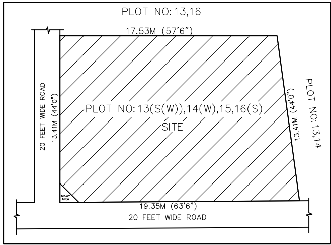
TOPO PLAN
