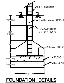
FOUNDATION DETAILS
