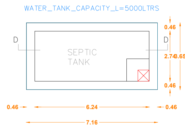
WATER_TANK_CAPACITY_L=5000LTRS
