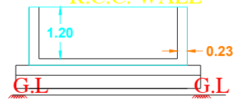
RWH_CAPACITY_L = 2000LTRS
