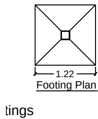
Footings
