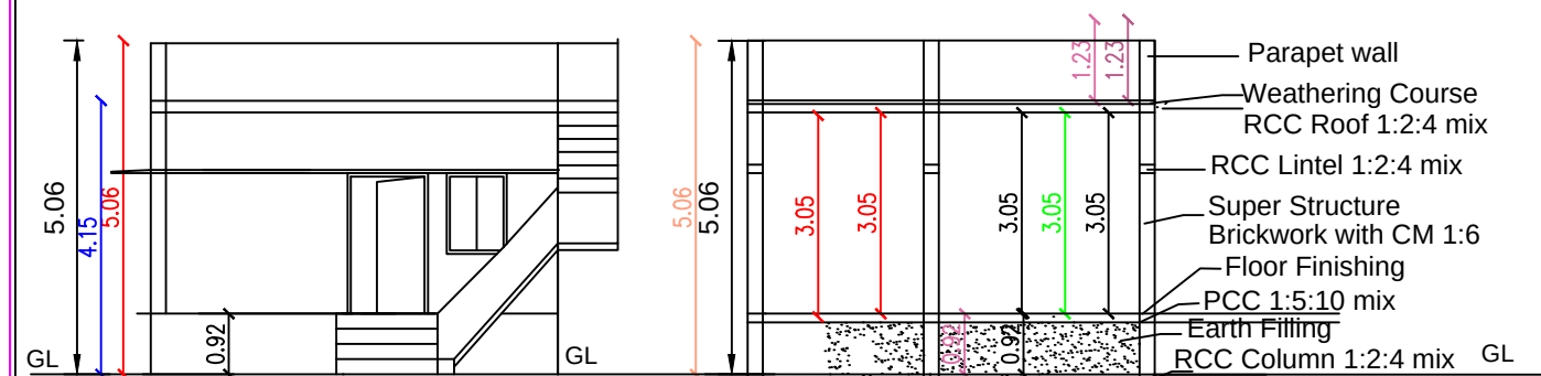
SECTION ON "VR"
