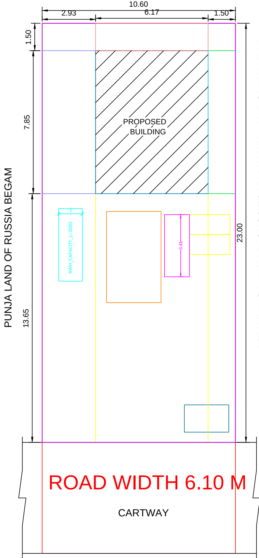
SITE PLAN
