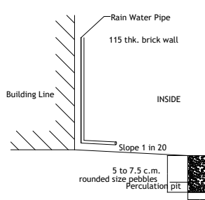
PERCOLATION PIT
