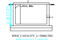
RAIN WATER HARVESTING:
