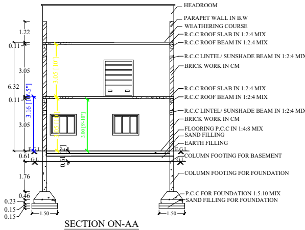
SECTION ON-AA
