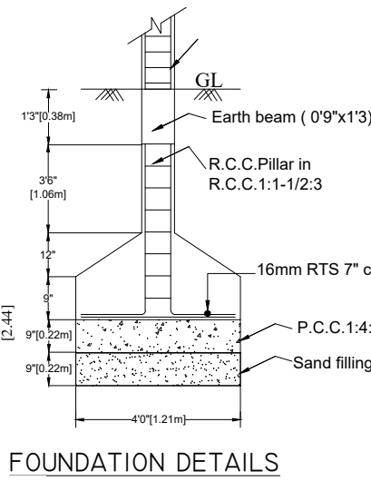
FOUNDATION DETAILS
