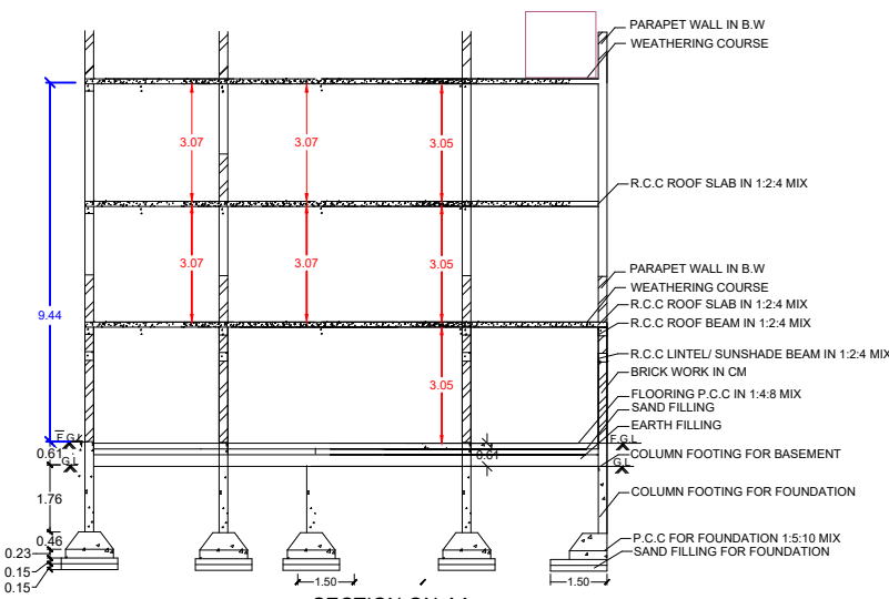
SECTION ON-AA
