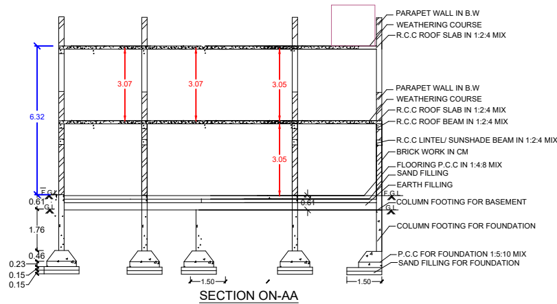
SECTION ON-AA
