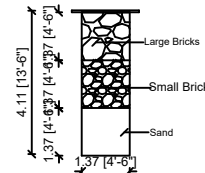
SECTION OF RAIN WATER
