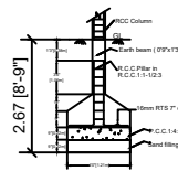
FOUNDATION DETAILS
