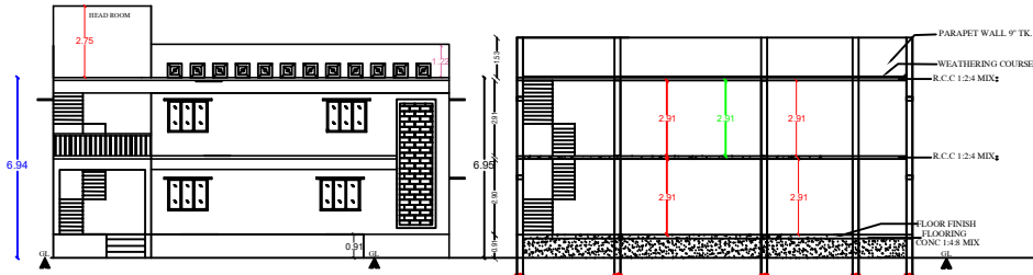
FRONT ELEVATION
