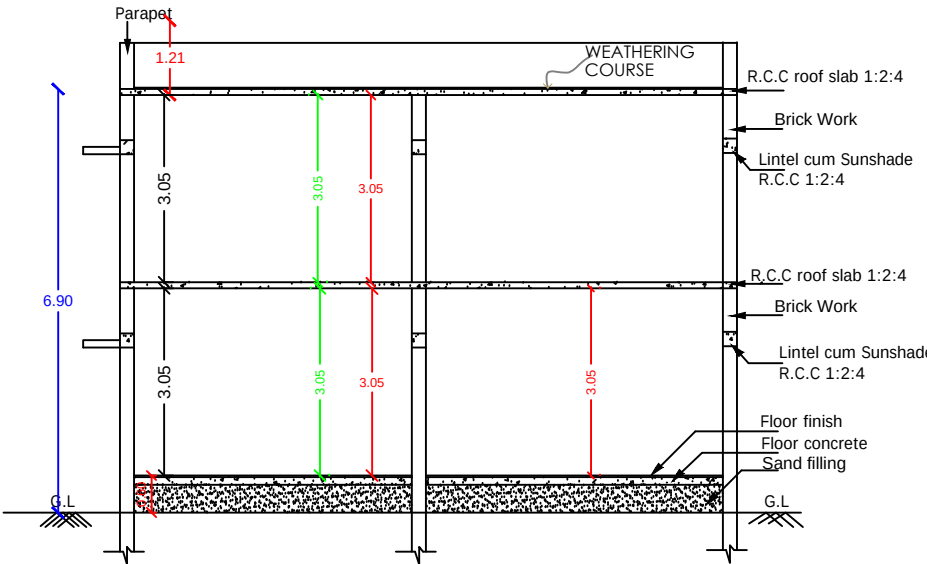
SECTION ON "A S"
