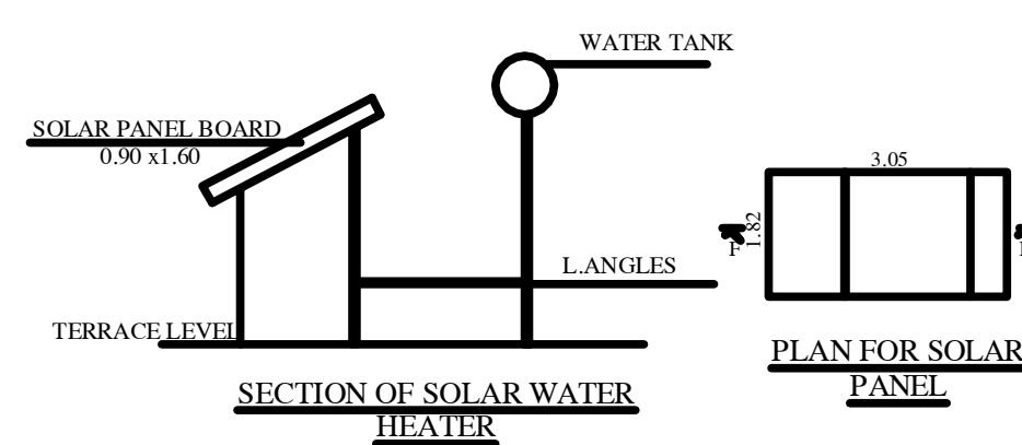
SECTION OF SOLAR WATER HEATER
