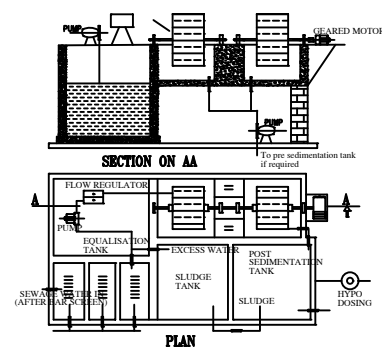
SEWAGE TREATMENT PLANT DETAILS
