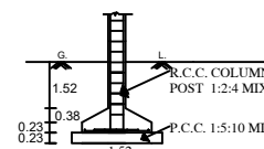
COLUMN POST DETAILS
