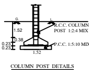
COLUMN POST DETAILS
