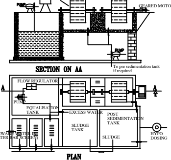
SEWAGE TREATMENT PLANT DETAILS
