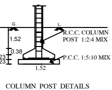
COLUMN POST DETAILS
