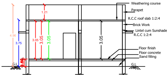
SECTION ON A
