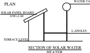
SECTION OF SOLAR WATER
