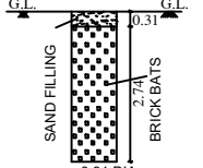
SECTION ON "A-B" A B 0.91 PI A
