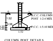
COLUMN POST DETAILS
